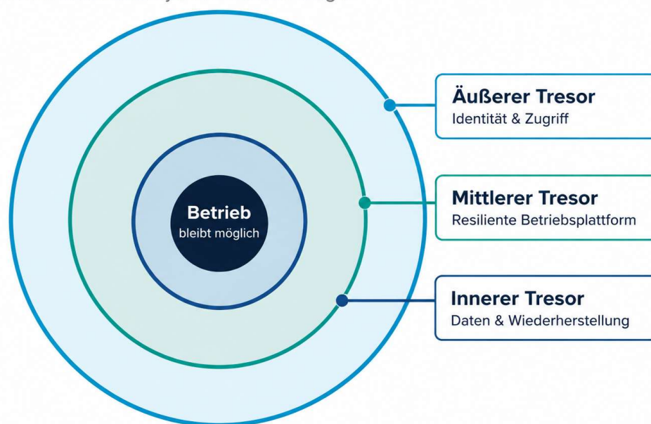
Abb. 4: Tresor-im-Tresor-Modell.
