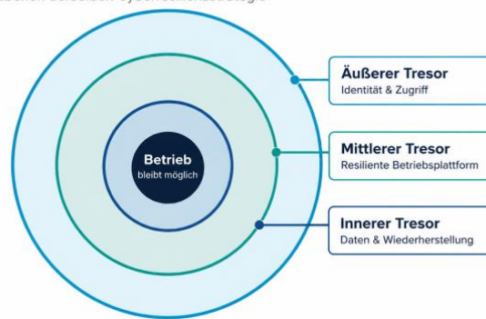
Abb. 4: Tresor-im-Tresor-Modell.
